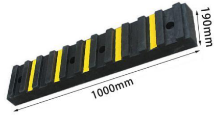
Size: 1000*190*80mm Weight: 13kg
