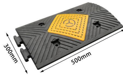
Size: 500*300*35mm Thickness: 35mm Weight: 3.25kg
