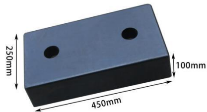
Size: 450*250*100mm Weight: 13kg
