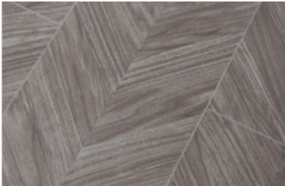
Single chip specifications: 1220 x 300 x 12mm MDF: 800/m 3
