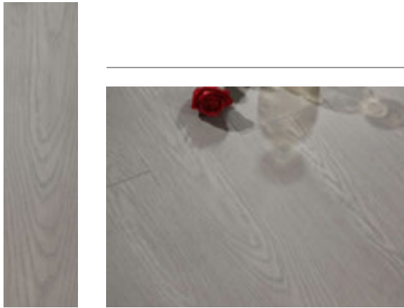
Single chip specifications: 1225 x 205 x 12mm MDF: 780/m 3
