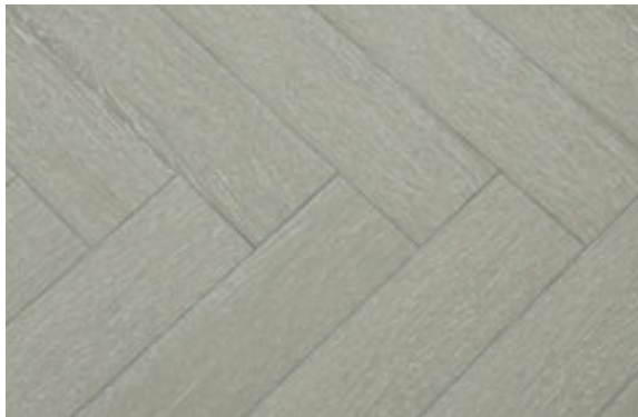
Single chip specifications: 608 x 105 x 12mm MDF: 800/m 3
