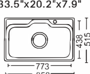
Size:850x515x200mm Inch:33.5"x20.2"x7.9"
