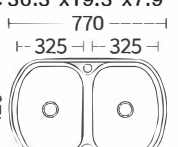
Size:770x490x200mm Inch:30.3"x19.3"x7.9"
