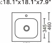
Size:460x460x200mm Inch:18.1"x18.1"x7.9"
