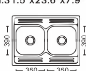
Size:800x600x200mm Inch:31.5"x23.6"x7.9"
