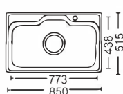
Size:850x515x200mm Inch:33.5"x20.2"x7.9"
