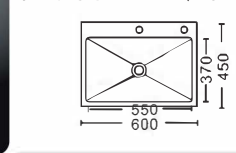
Size: 600x450x(200~230)mm Inch: 23.6"x17.7"x(7.9"-9")
