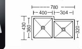
Size: 780x430x(200~230)mm Inch: 30.7"x16.9"x(7.9"-9")
