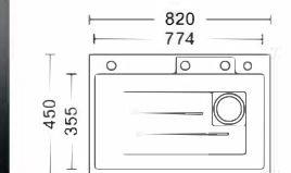
Size: 820x450x220mm Inch: 32.2"x17.7"x8.7"
