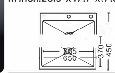
Size: 650x450x(200~230)mm Inch: 25.5"x17.7"x(7.9"-9")
