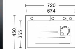
Size: 720x450x220mm Inch: 28.3"x17.7"x8.7"
