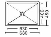
Size:680x450x(200~230)mm Inch:26.7"x17.7"x(7.9"-9")
