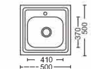
Size:500x500(145~200)mm Inch:19.6"x19.6"x(5.7"~7.9")
