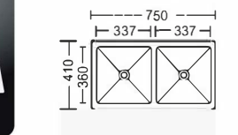
Size: 750x410x(200~230)mm Inch: 29.5"x16.1"x(7.9"-9")
