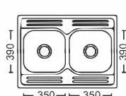
Size:800x600x200mm Inch:31.5"x23.6"x7.9"
