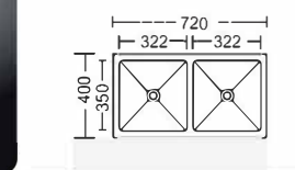
Size: 720x400x(200~230)mm Inch: 28.3"x15.7"x(7.9"-9")
