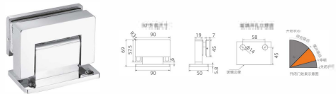
单向缓冲 90°防水铰链 Soft Close Waterproof Hinge (Single Side Opening)
