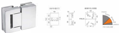
单向缓冲 180°防水铰链 Soft Close Waterproof Hinge (Single Side Opening)
