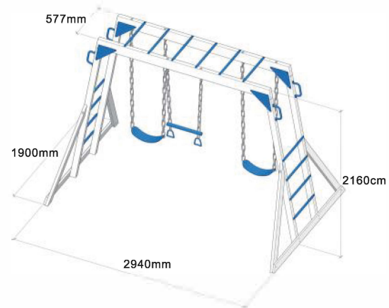
Size:2940*1900*2160mm
