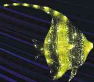
LED number: 145LEDs Size: W89 x H55cm Weight: 5.7kg Voltage: 24VDC / 100-130VAC / 220-240VAC
