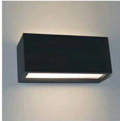
LED 12Wx1 COB / 960Lm Ra: >80 PF: 0.85 Working temperature: -15°C~50°C
