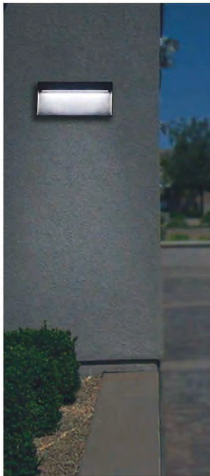
LED 12Wx1 COB / 960Lm Ra: >80 PF: 0.85 Working temperature: -15°C~50°C
