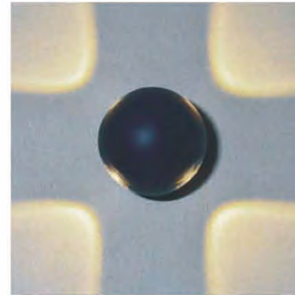
LED 3Wx4 COB / 1080Lm Ra: >80 PF: 0.85 Working temperature: -15°C~50°C
