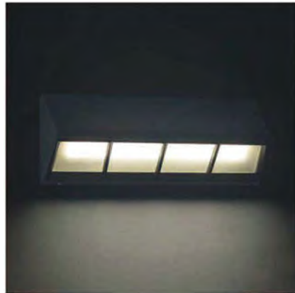
● 24W COB / 1920Lm Ra: >80 PF: 0.85 Working temperature: -15°C~50°C
