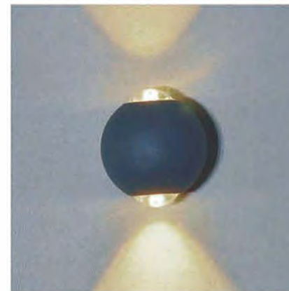
LED 3Wx2 COB / 540Lm Ra: >80 PF: 0.85 Working temperature: -15°C~50°C
